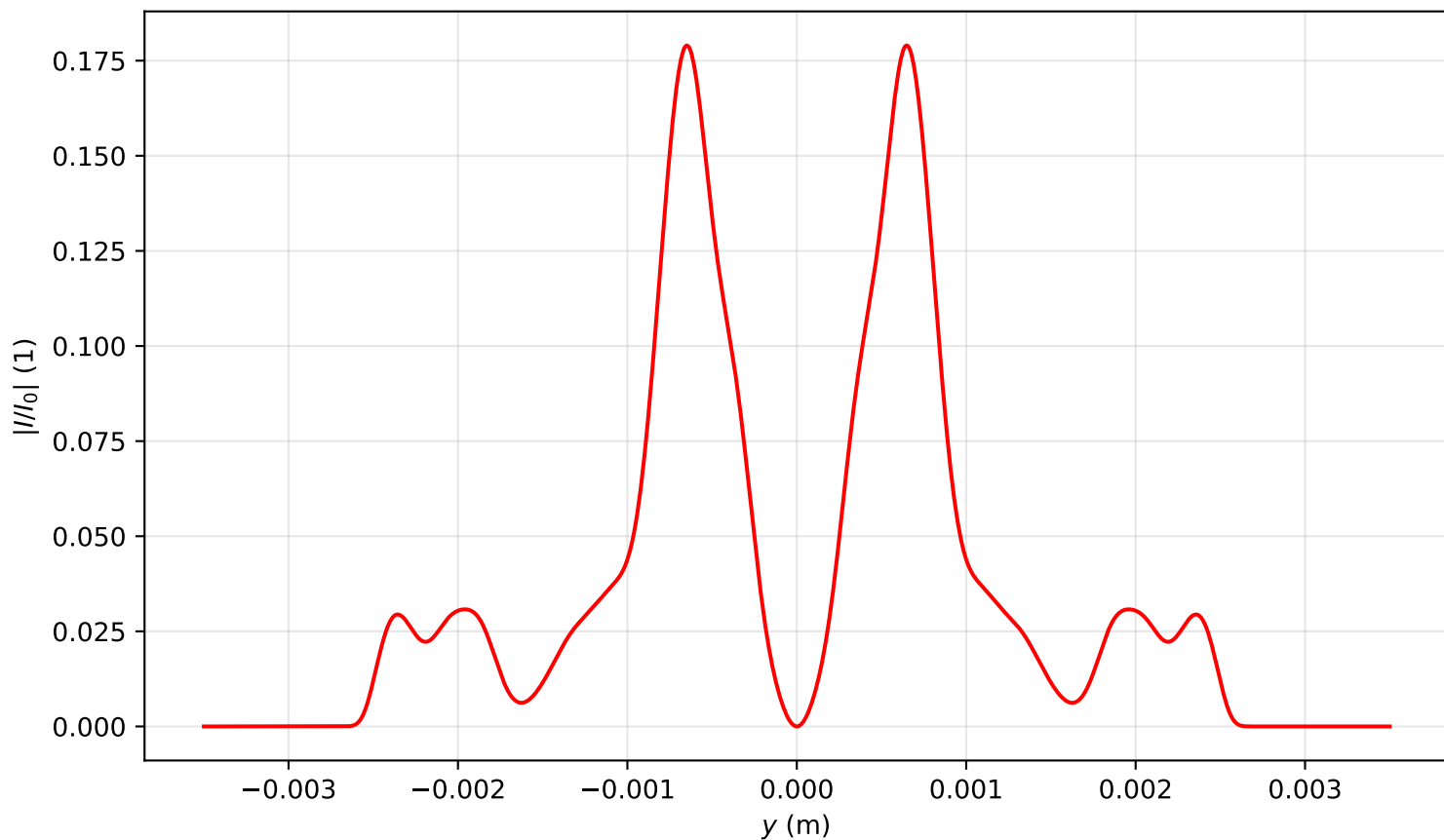
Intensity profile I(x=0, y, z=3.503)/I_0 , Pin=9.0Pcr, artificial time
